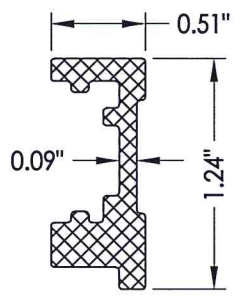
10 LOCK STILE REINFORCEMENT
