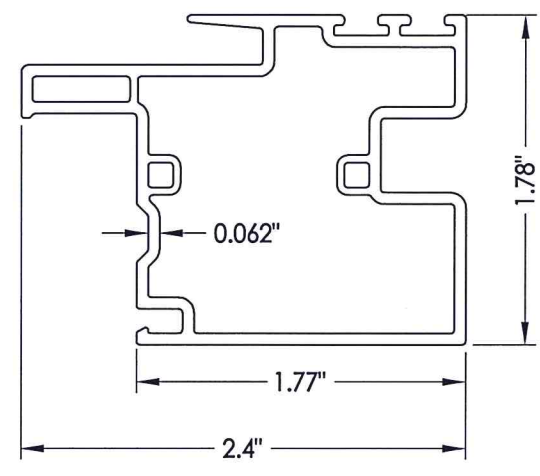
6 MEETING STILE
