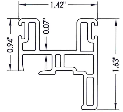
5 TOP RAIL
