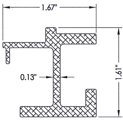
9 MEETING STILE REINFORCEMENT
