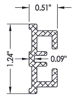
13 HANDLE STILE REINFORCEMENT
