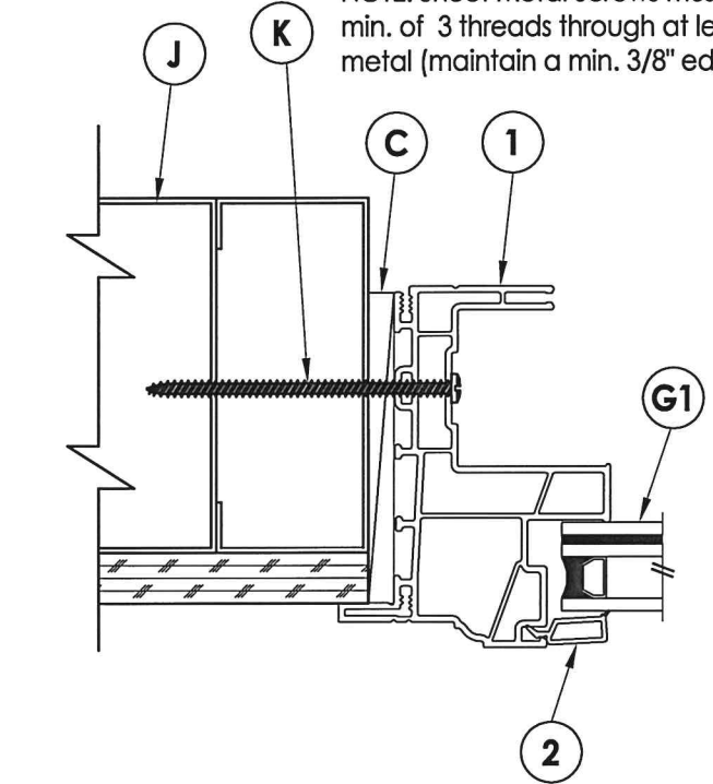
4 HORIZONTAL CROSS SECTION 2 Metal Stud Construction
