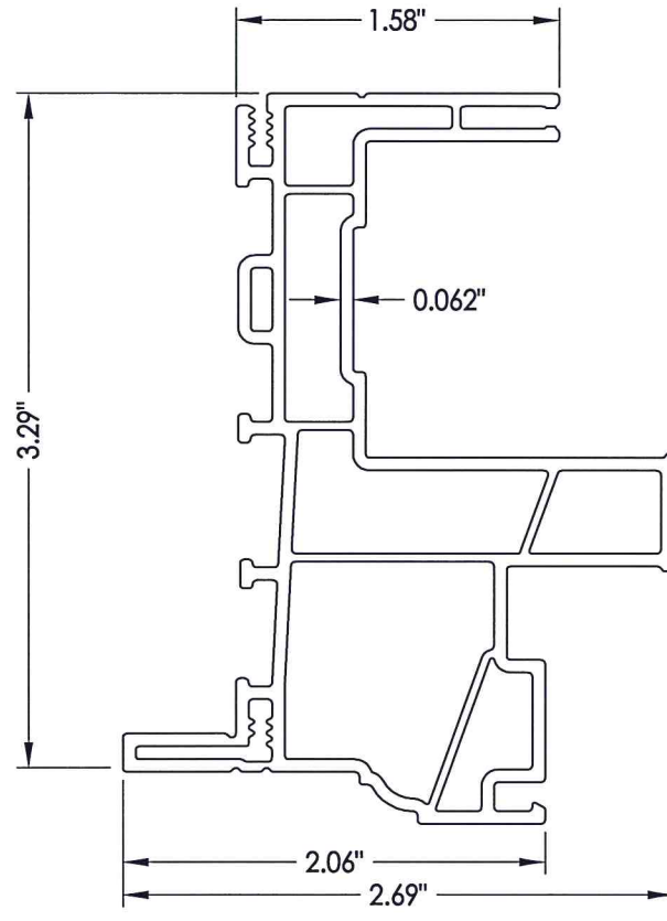
1 FRAME
